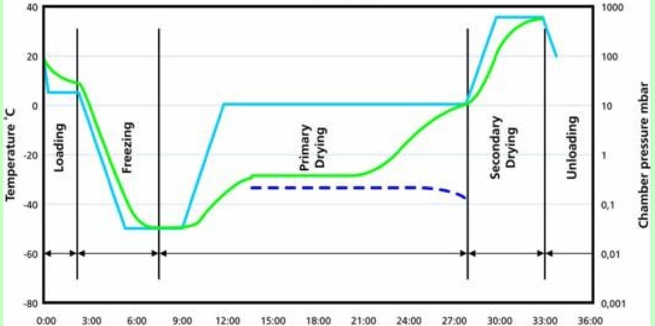
Freeze Drying Cycle
