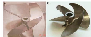
Fig. 43 (a) An AREC "elephant ear" impeller (used down-pumping); (b) Hayward Tyler up-pumping B2 hydrofoil
