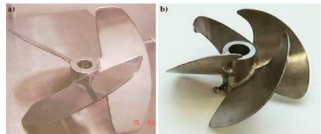
Fig. 13 (a) An ARBC "elephant ear" impeller (used down-pumping); (b) Hayward Tyler up-pumping B2 hydrofoil
