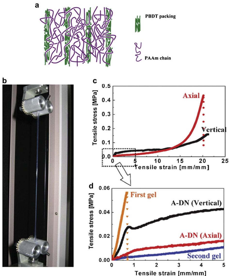
Fig. 12. (a) Schematic representation of a possible well-ordered structure in the anisotropic double network (A-DN) gel. High extensibility of the A-DN gel containing 1wt % PBDT: (b) Photograph demonstrating the tensile capability of the A-DN gel that can elongate to over 22 times of its original length. (c) Tensile stress-strain curves of A-DN gel in axial and vertical directions. (d) Enlarged curves at the initial elongation of the A-DN gel and corresponding two individual single network gels (PBDT SN gel and PAAm SN gel). Reproduced with permission from the literature [39].
