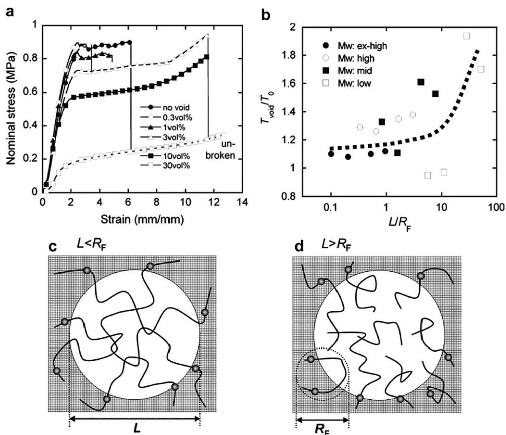
Fig. 9. (a) Stress-strain curves of void-DN gels with various volume fraction of the void (void diameter, L = 200 nm). The initiator concentration of the second network was 0.02 mol % and M_w was 3.0 \times 10^6 g/mol. The tensile velocity was 100 mm/min. The tensile strength was much larger than R_F (a line is guide for eyes). T_{void} and T_0 is the tearing energy of the void and void-free DN gel, respectively. (b) Relative tearing energy ( T_{void}/T_0 ) dependence on L/R_F ( R_F : Flory radius of the PAAm). T_{void}/T_0 increased twice when the void diameter L was much larger than R_F (a line is guide for eyes). (c) In the case of L < R_F , the void is bridged by several PAAm chains via the covalent bonds between the two networks. (d) If L > R_F , PAAm chains are relatively too short to bridge the void structure, thus, the void can form "true" hollow structure. The mesh around the void denotes PAAm network and the solid chains denote PAAm. Reproduced with permission from the literature [37].
