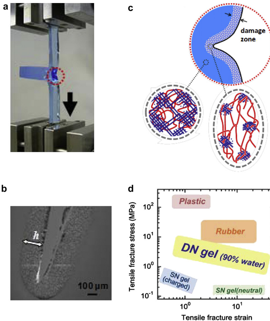
Fig. 2. (a) Image of the tearing test of double network (DN) gel. (b) Image of the crack tip of the DN gel after tearing observed under a color three-dimensional violet laser scanning microscope. (c) Illustration of network structure of the DN gel at the crack front and damage zone. (d) Comparison of the toughness of the DN gel with various polymer materials. Reproduced with permission from the literature [26,55].
