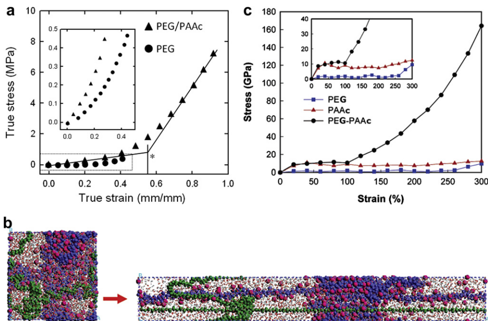
Fig. 5. (a) True compressive stress versus true strain plots for (a) PEG single network gel and (b) PEG/PAAc DN gel. The molecular weight of PEG is 4600 Da in both gels. The intersection (*) between the initial and final tangents to the stress-strain curve of PEG/PAAc defines the critical strain ( \epsilon_{crit} ) for strain hardening in each IPN. (b) Molecular dynamic simulations of PEG/PAAc DN hydrogel system at normal state and elongated state (300%). (c) Stress-strain curves of PEG, PAAc, and PEG/PAAc hydrogels from uniaxial elongation simulations. Reproduced with permission from the literature [45,47].
