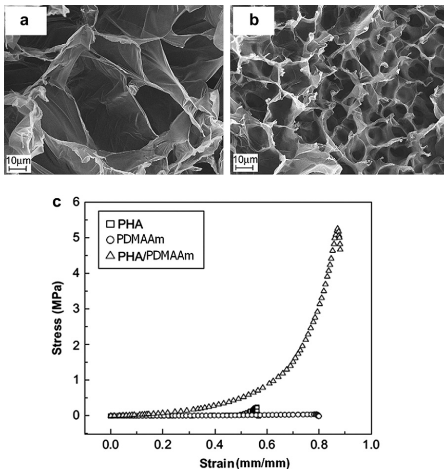
Fig. 6. Representative SEM images for the (a) PHA and (b) PHA/PDMAAm. (c) Stress-strain profiles for the PHA, PDMAAm, and PHA/PDMAAm hydrogels under uniaxial compression. Reproduced with permission from the literature [50].
