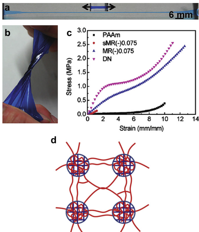
Fig. 10. Microgel-reinforced particle double network gel (MR gel) film, dyed by Alcian Blue, subject to high elongation from the free-standing state to the stretching state of strain = 11 mm/mm (a) and torsion (b). (c) Comparison of tensile stress-strain curves of PAAm, sMR, MR, and conventional DN gels. (d) Schematic representation of the network structure of MR gel. Reproduced with permission from the literature [38].
