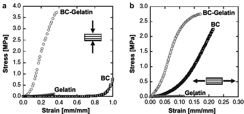
Fig. 4. Compressive (a) and tensile (b) stress-strain curves of bacterial cellulose (BC), gelatin, BC/gelatin DN gels. The compression and elongation were performed in perpendicular to and along with the stratified direction of BC and BC/gelatin DN gels, respectively. Concentration of gelatin in feed: 30wt%. EDC concentration: 1 M. Reproduced with permission from the literature [35].
