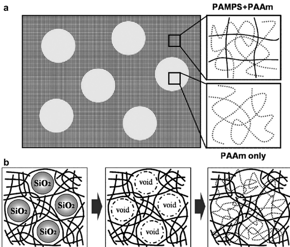
Fig. 8. (a) The structure model and (b) the synthesizing pathway of void-DN gels with hard PAMPS/PAAm body and soft spherical PAAm void, which are obtained by polymerizing PAAm (dotted chain) in the presence of PAMPS gels (solid chain) containing hollow spherical structure. Reproduced with permission from the literature [37].
