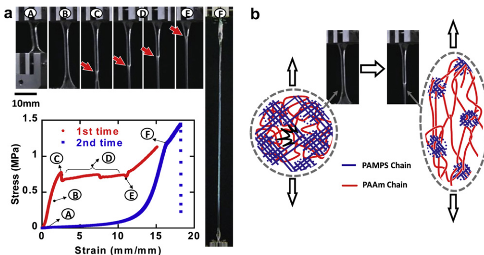
Fig. 1. (a) Loading curves of PAMPS/PAAm double network (DN) gel under uniaxial elongation at a rate of 0.13 \text{ s}^{-1} , and images demonstrating the necking process. The insert letters represent the correspondence between the images and the data points in the loading curves. (b) Illustration of the network structure of the DN gel before and after necking. Above a critical stress, PAMPS network fractures into clusters that behave as a sliding cross-linker of PAAm. After necking DN gel becomes soft. Reproduced with permission from the literature [26].
