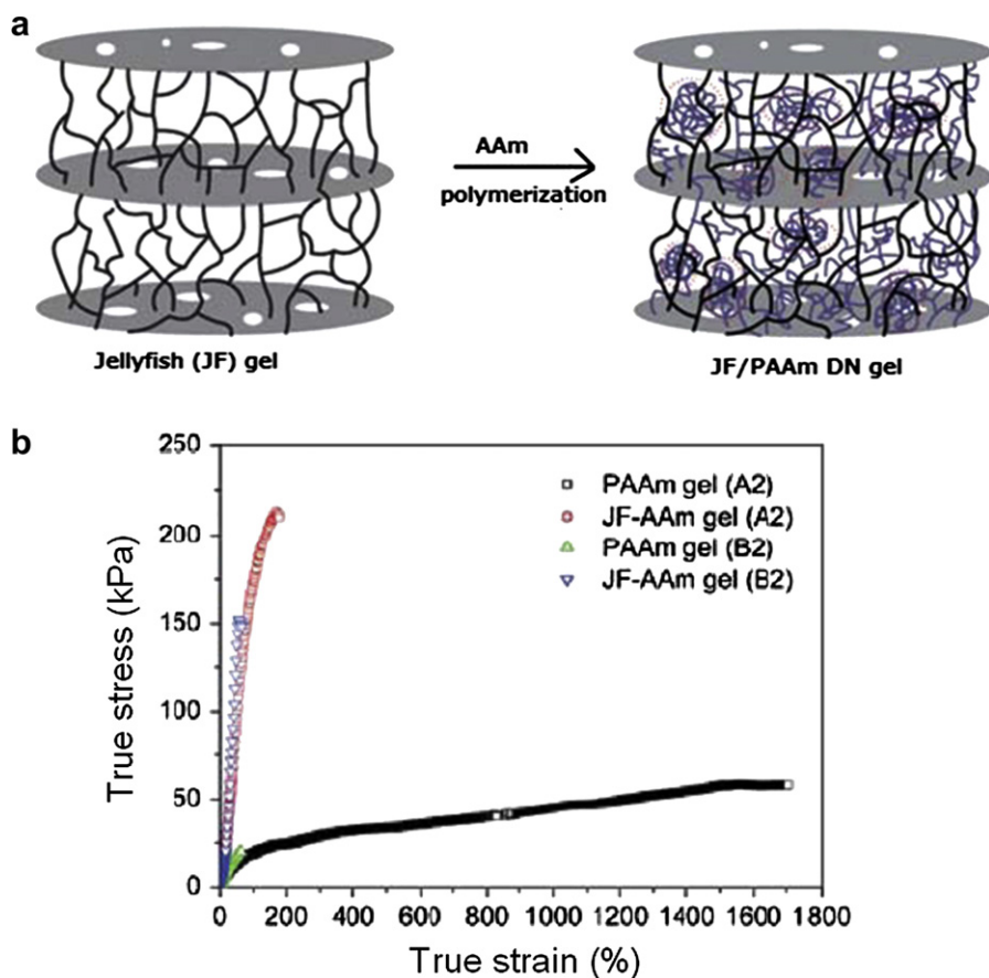
Fig. 7. (a) Schematic microstructures of jellyfish (JF) gel and JF/PAAm DN gel. (b) The typical tensile stress-strain curves of JF/PAAm and PAAm gels. Reproduced by permission of the Royal Society of Chemistry [51].
