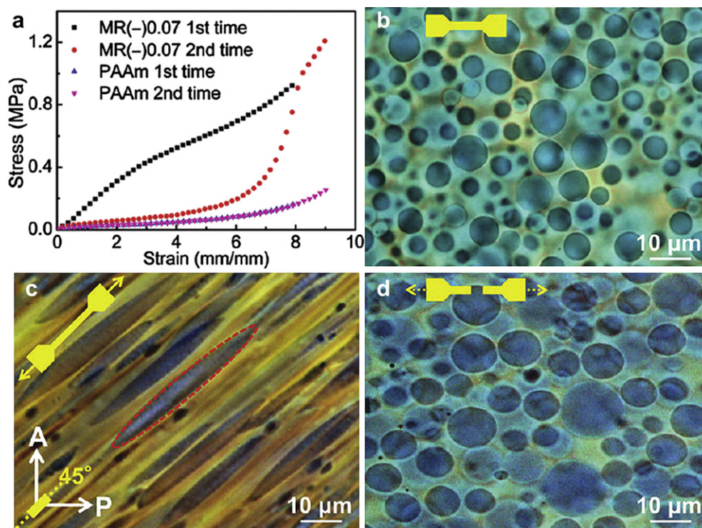
Fig. 11. (a) Hysteresis in stress-strain curves of microgel reinforced particle double network gel (MR gel) and the PAAm gel. The first and the second elongation are stopped at the strain = 8 mm/mm and strain = 9 mm/mm, respectively. (b) Optical microscopy image of MR gel film at the free-standing state. (c) Real-time tensile observation of MR gel film at the strain of 4 mm/mm by a polarizing microscope, equipped with the crossed polarizers and the 530 nm tint plate. The sample was stretched 45° against the polarizers. The red dashed line indicates the deformed microgel. (d) Residual strain observation of re-swollen MR gel film after tensile fracture by an optical microscope. The elliptical shape of the microgels indicates the occurrence of the internal fracture after elongation. MR gel film is dyed by Alcian Blue for (b–d). Reproduced with permission from the literature [38].
