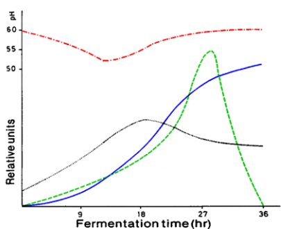
The kinetics of the acetone-butanol fermentation (Spivey, 1978). — solvent, — gas production, - - - pH value
