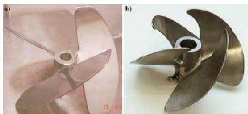
Fig. 13 (a) An ABC 'depart car' impeller (used down-pumping); (b) Hayward Tyler up-pumping B2 hydrofoil
